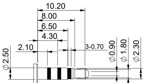
(Ø2.50mm 4 POLE PLUG DETAIL DRAWING)
