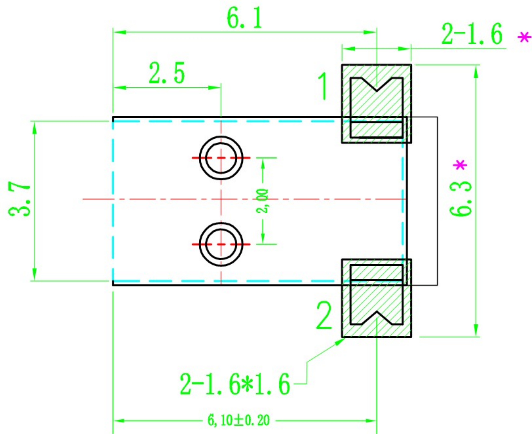
PCB LAYOUT TOP VIEW
