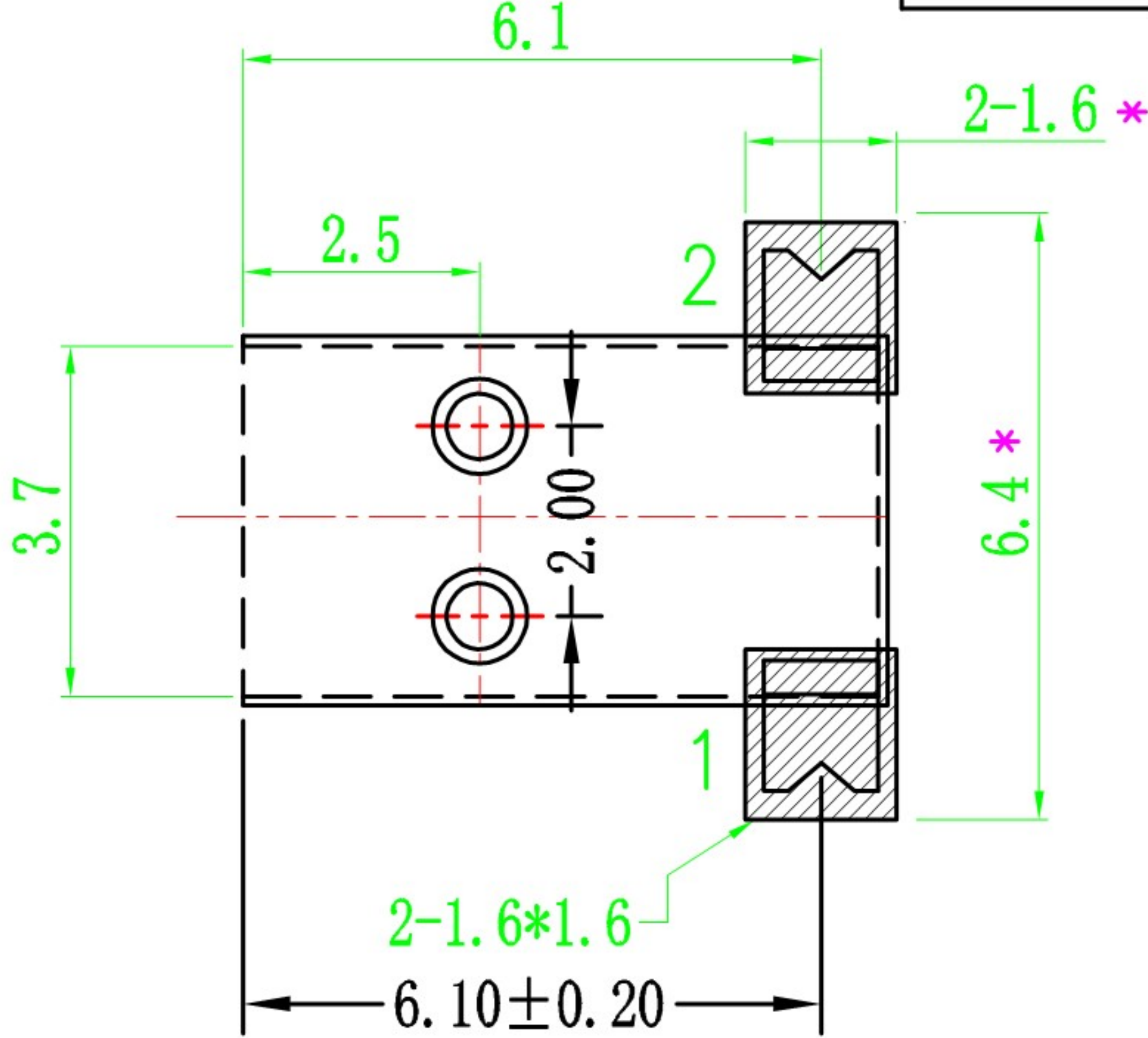
PCB LAYOUT TOP VIEW
