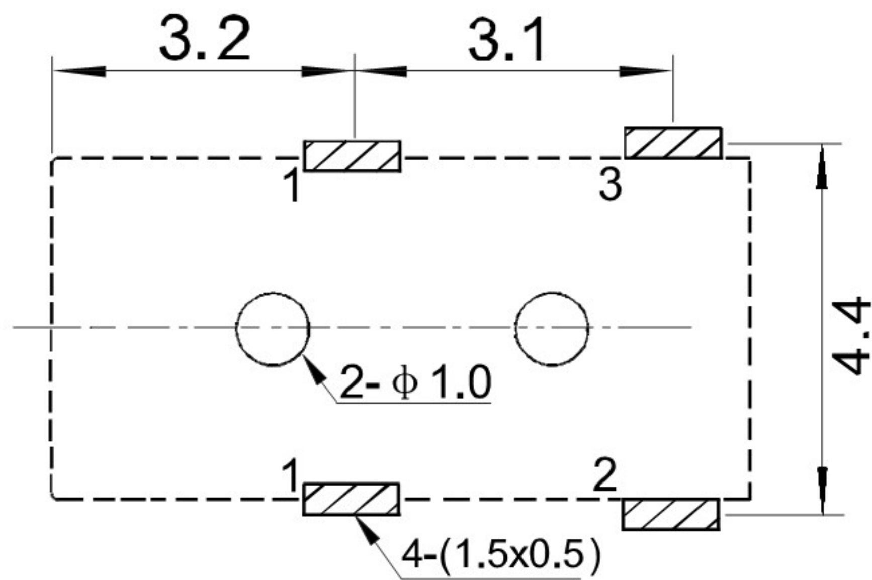
Pad Layout
