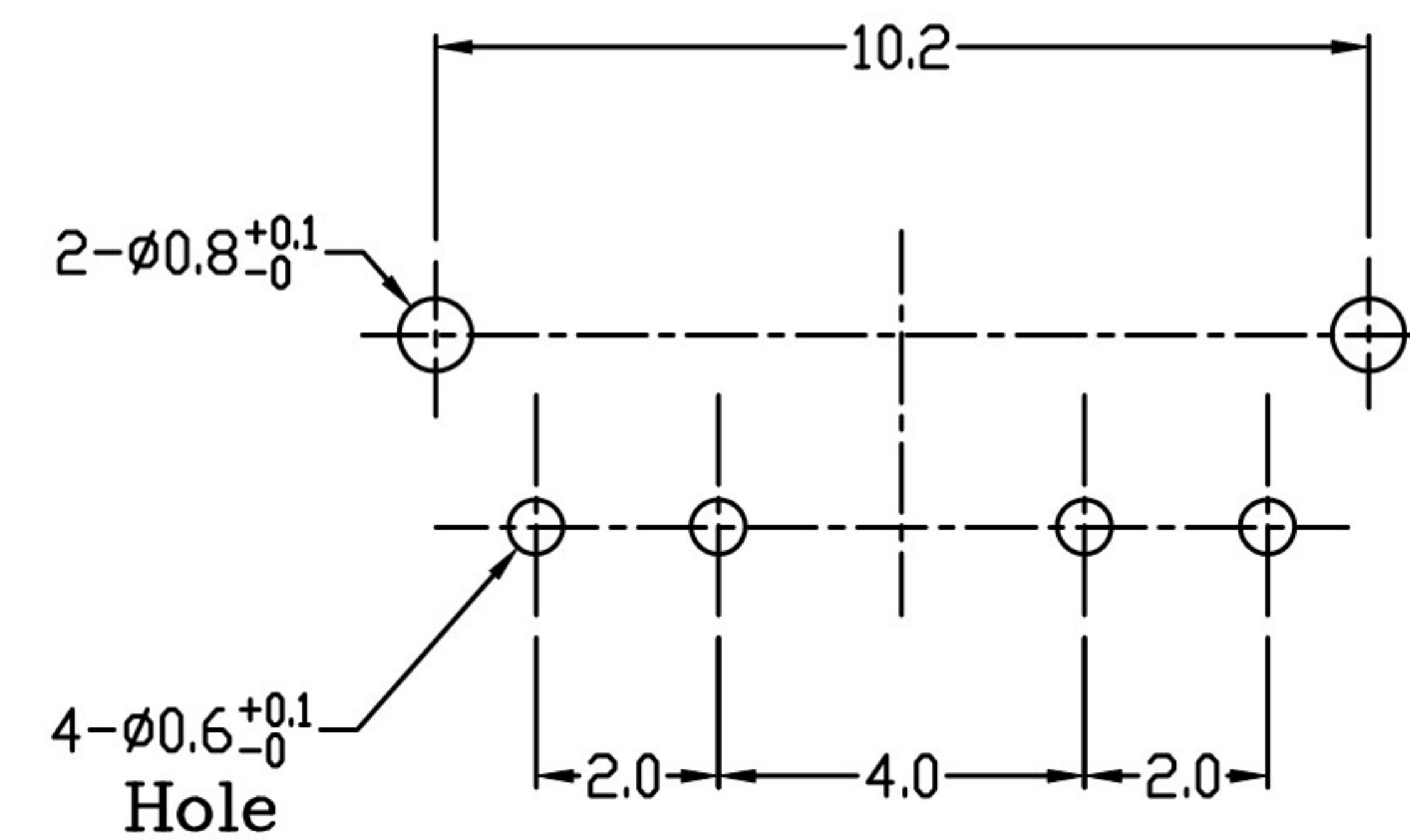
P.C. BOARD LAYOUT
