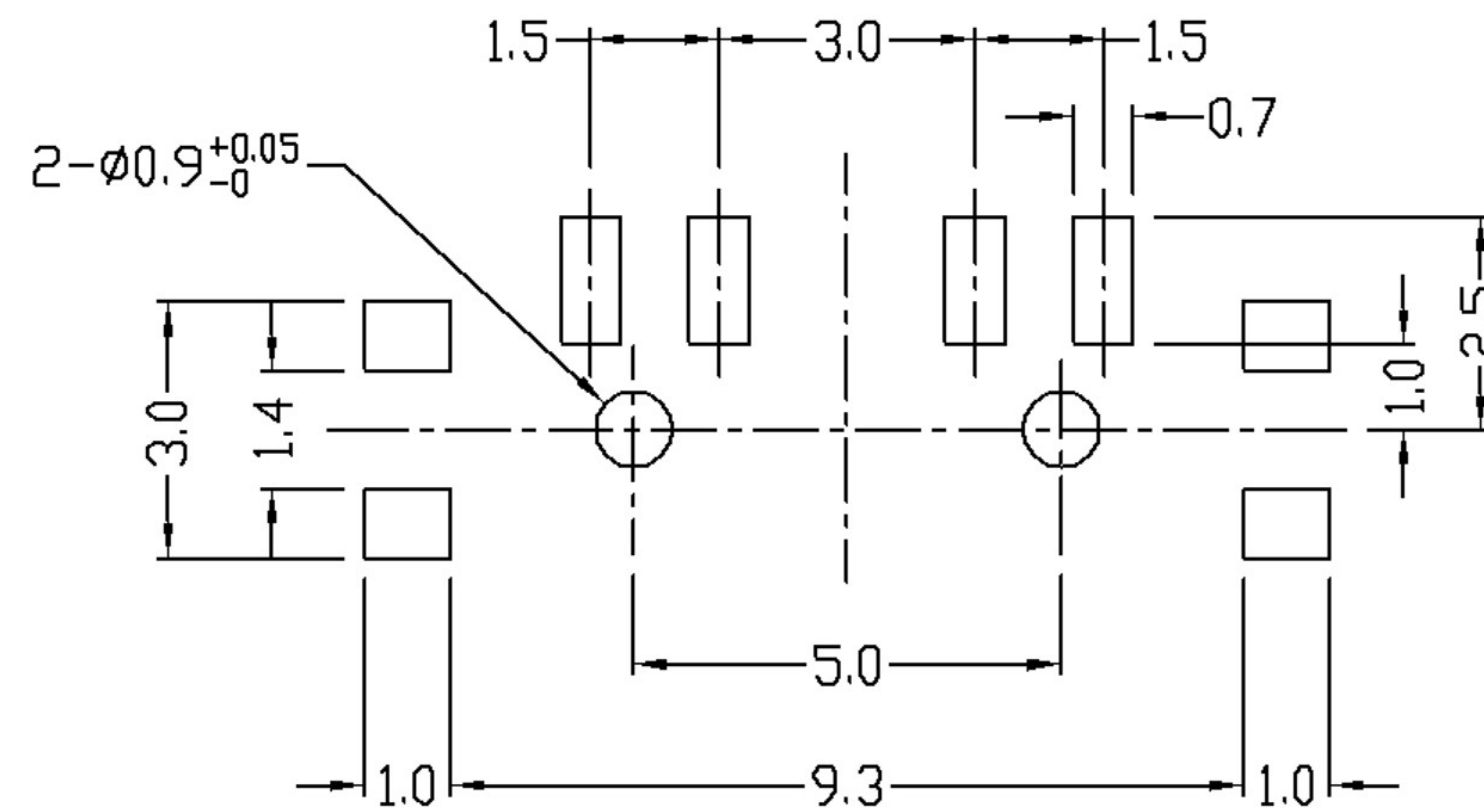
P.C. BOARD LAYOUT VIEW A
