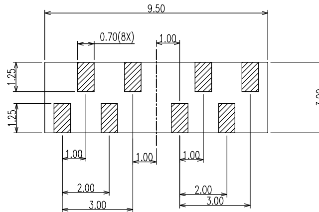
RECOMMENDED FLEX LAYOUT
