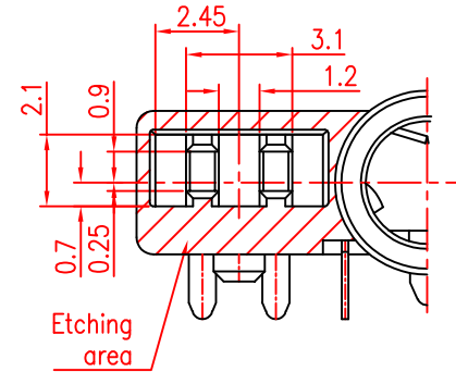
Detail of the connector (s=4:1)
