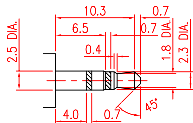
MATE PLUG
