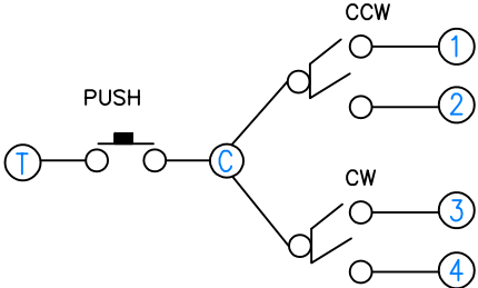
CIRCUIT
