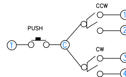
CIRCUIT
