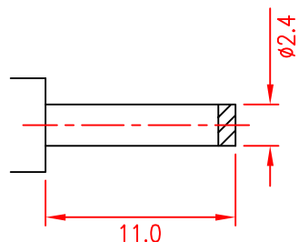
MATE PLUG
