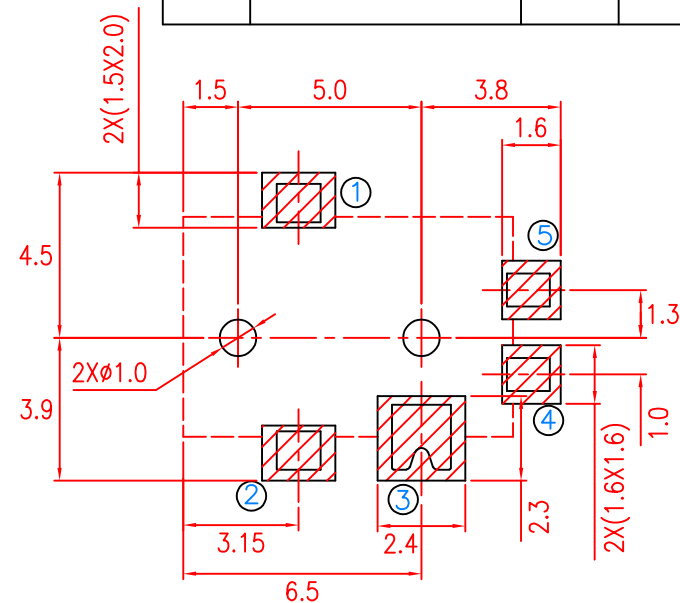
P.C.B LAYOUT BOTTOM VIEW
