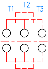
CIRCUIT
