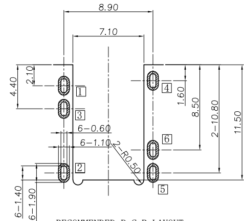
RECOMMENDED P.C.B LAYOUT TOP VIEW (TOLRANCE:±0.05)
