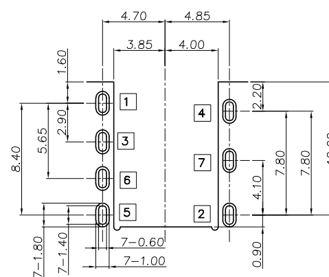
RECOMMENDED P.C.B LAYOUT (t=1.0mm) TOP VIEW (TOLRANCE: ±0.05)
