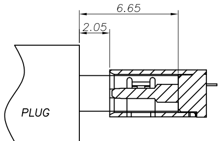
AFTER MATING
