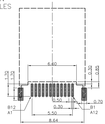
RECOMMENDED P.C.B. LAYOUT (T:0.8mm) TOLERANCE UNSPECIFIED ±0.05mm
