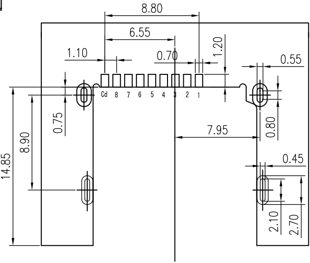
RECOMMENDED P.C.B HOLE LAYOUT COMPONENT SIDE VIEW(TOLERANCE: \pm 0.05 )
