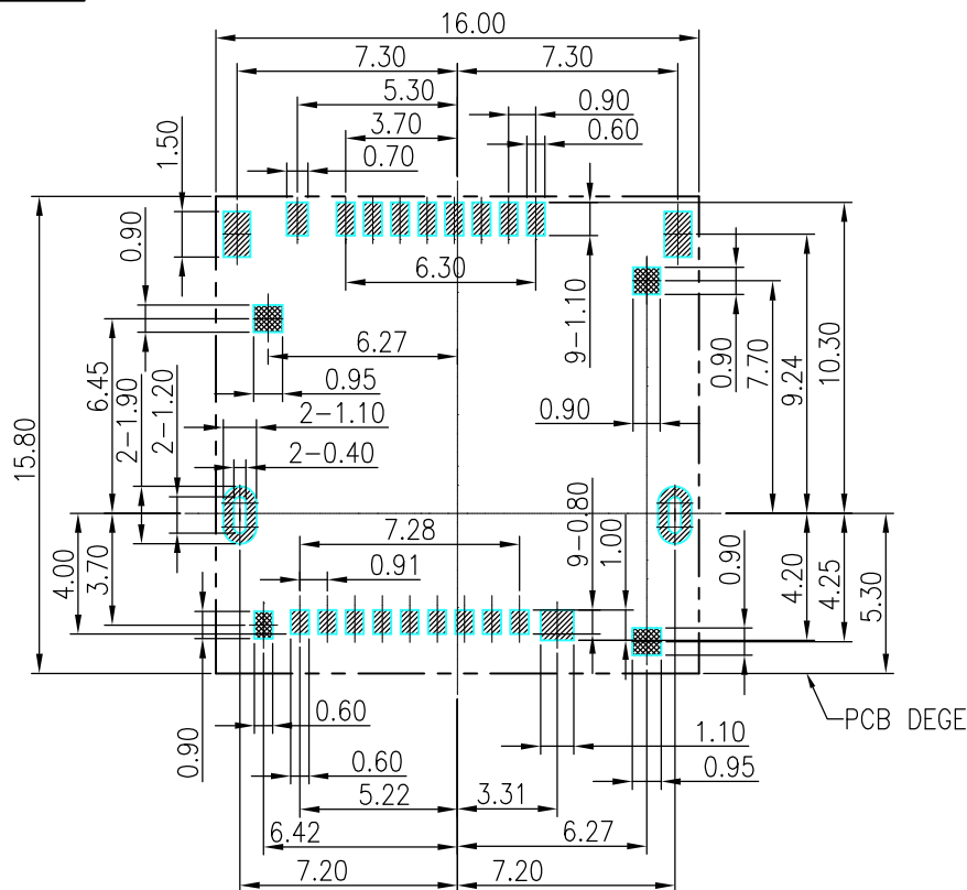
RECOMMEENDED P.C.B LAYOUT TOP VIEW(TOLERANCE+/-0.05)
