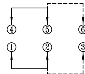
SCHEMATIC (NON-SHORTING)
