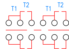
CIRCUIT
