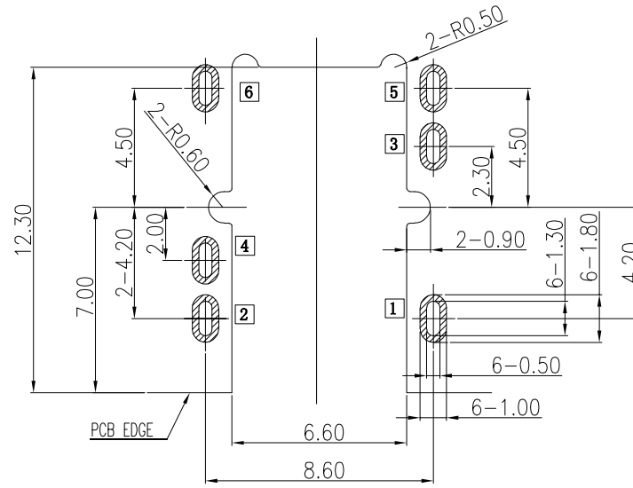
RECOMMENDED P.C.B. LAYOUT TOP VIEW (TOLRANCE:±0.05)
