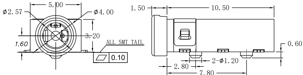
( \phi 2.50mm 4 POLE PLUG DETAIL DRAWING)
