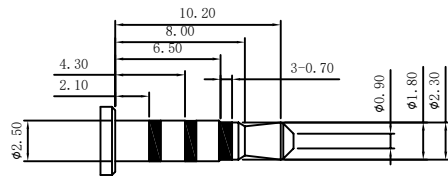
( \phi 2.50mm 4 POLE PLUG DETAIL DRAWING)
