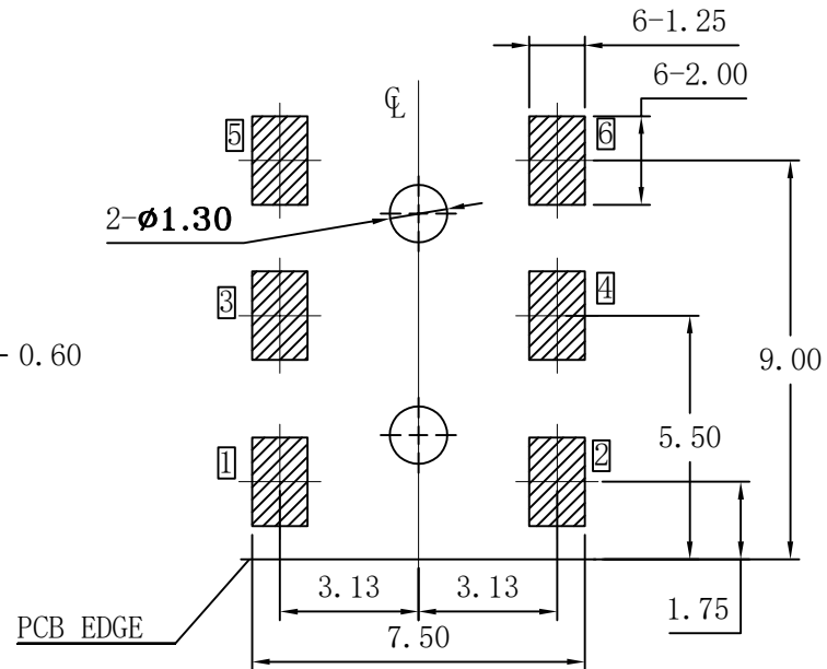
RECOMMENDED PCB LAYOUT (TOP VIEW) (GENERAL TOLERANCE \pm 0.05 )
