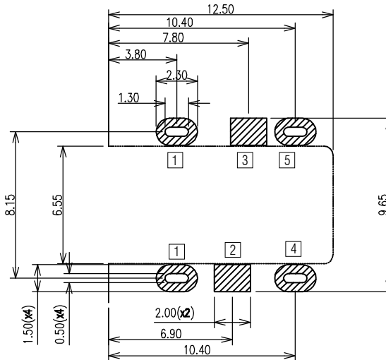
RECOMMEND PAD LAYOUT
