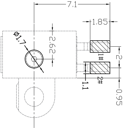
P.C.B MOUNTING PATTERN DIMENSION
