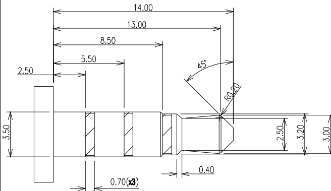
THE RECOMMENDED MATING AUDIO PLUG 3.50mm 4 POLE PLUG
