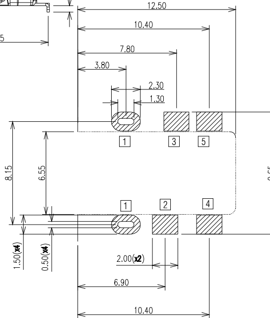
RECOMMEND PAD LAYOUT
