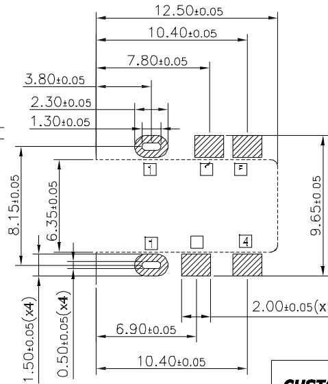
RECOMMEND PAD LAYOUT
