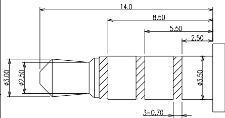
(Ø3.50mm 4 POLE PLUG DETAIL DRAWING)
