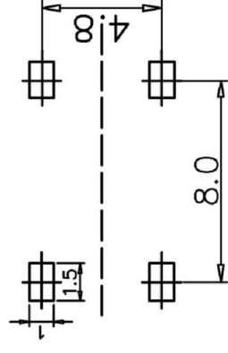
PCB LAYOUT MOUNTING PATTERN
