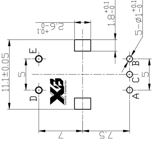
P.C.B MOUNTING HOLE DETAIL
