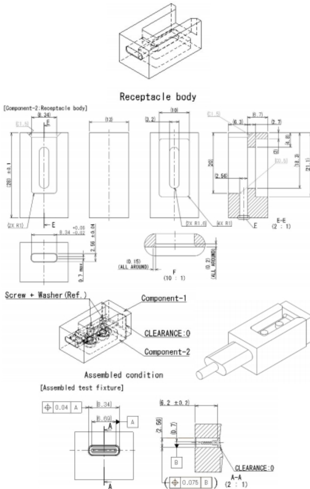
Figure D-3. Wrenching Strength Test Fixture
