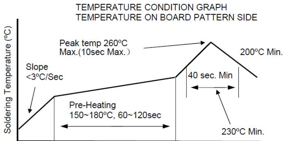
Fig 1 – Temperature profile of Reflow Soldering at 260^{\circ}\text{C} Max.
