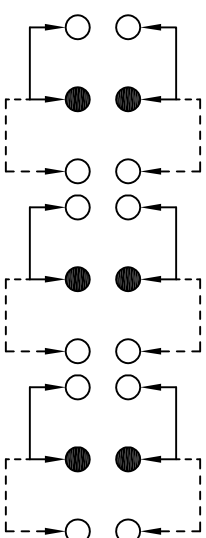
SCHEMATIC (NON-SHORTING)
