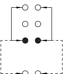
SCHEMATIC (NON-SHORTING)
