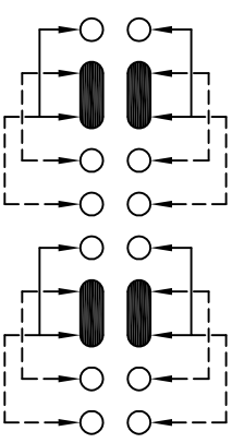
SCHEMATIC (SHORTING)
