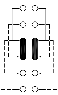
SCHEMATIC (SHORTING)
