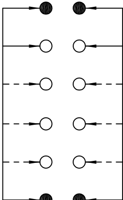
SCHEMATIC (NON-SHORTING)
