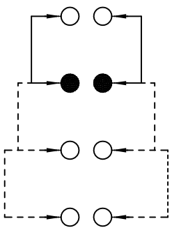
SCHEMATIC (NON-SHORTING)
