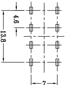
P.C.B LAYOUT BOTTOM VIEW
