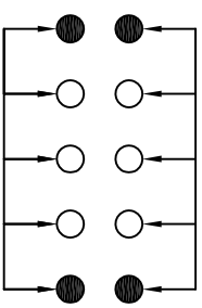
SCHEMATIC(NON-SHORTING)
