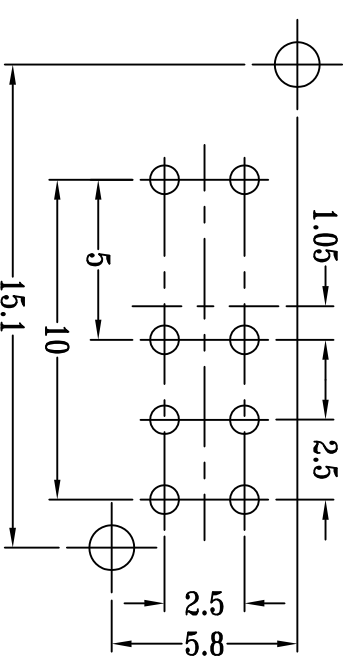
P.C.B LAYOUT BOTTOM VIEW
