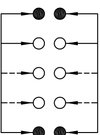
SCHEMATIC (NON-SHORTING)
