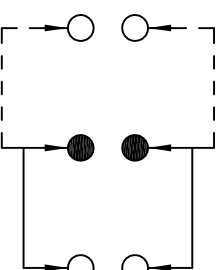
SCHEMATIC (NON-SHORTING)
