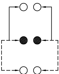
SCHEMATIC (NON-SHORTING)
