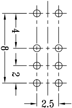
P.C.B LAYOUT BOTTOM VIEW
