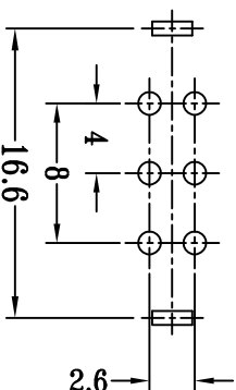
P.C.B LAYOUT BOTTOM VIEW
